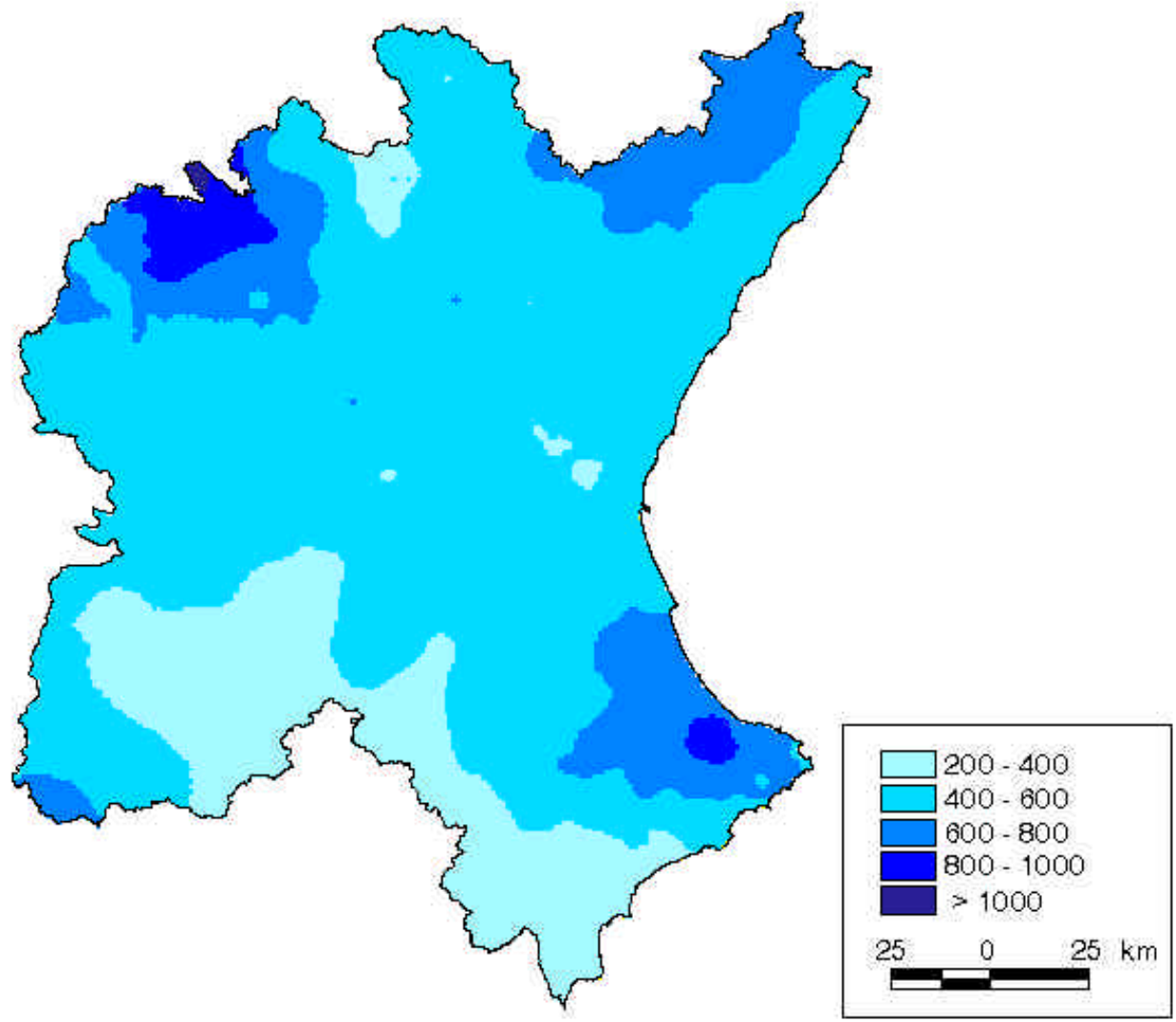
Mean annual rainfall (mm)
