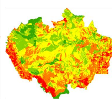
Drought Vulnerability
