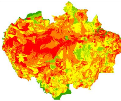
Flood Vulnerability
